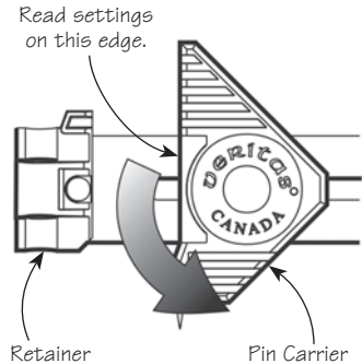
Figure 1: Compass position.
