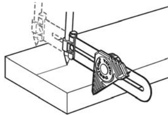
Figure 3: Center marking.
